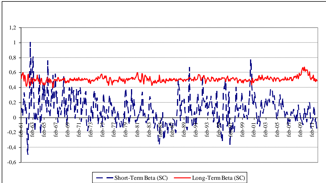
Panel B: Average Short- and Long-Term Betas across 40 Test Assets Sorted by Book-to-Market, Size, Momentum and Long-term Reversals with Default: February 1961-December 2011
