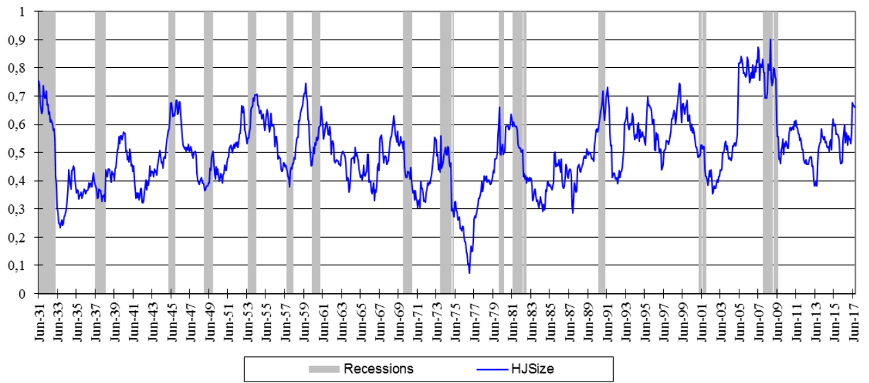
Volatility (bound) of the stochastic discount factor 10 US size-sorted portfolios with five years of overlapping data from January 1927 to August 2017, and the average risk-free rate for each sub-period
