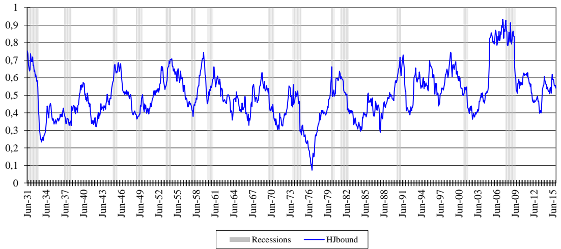
Volatility (bound) of the stochastic discount factor U.S. size-sorted portfolios with five years of overlapping data from January 1927 to December 2015, and the average level of the interest rate for each sub-period
